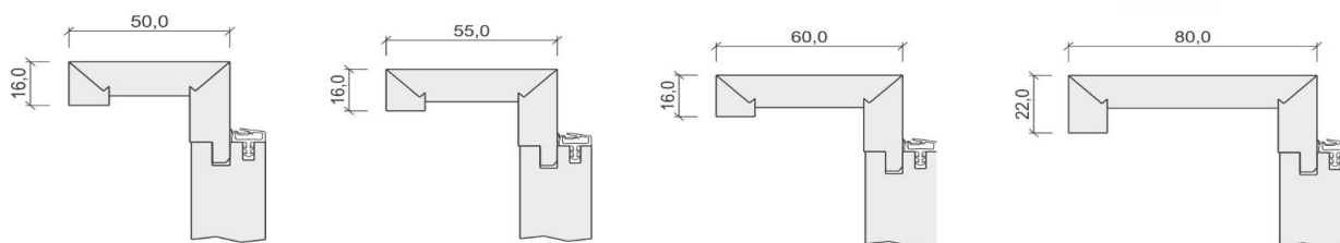
FU-EC 50/16 mm
