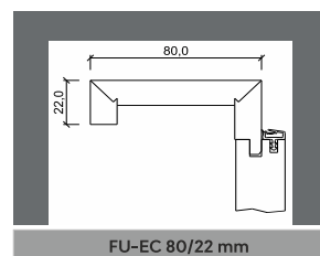
FU-EC 80/22 mm
